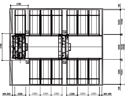
SHUTTLE SYSTEM
