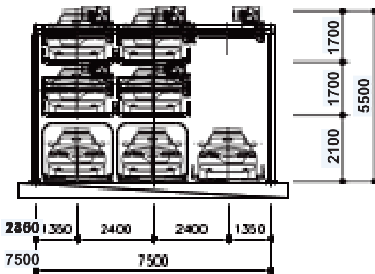
PUZZLE PARKING
